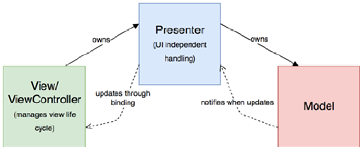
Fig: Model-View-Presenter
